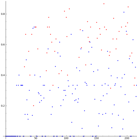
FIGURE 1. \frac{N_p}{s_p} for p < 10000 .
