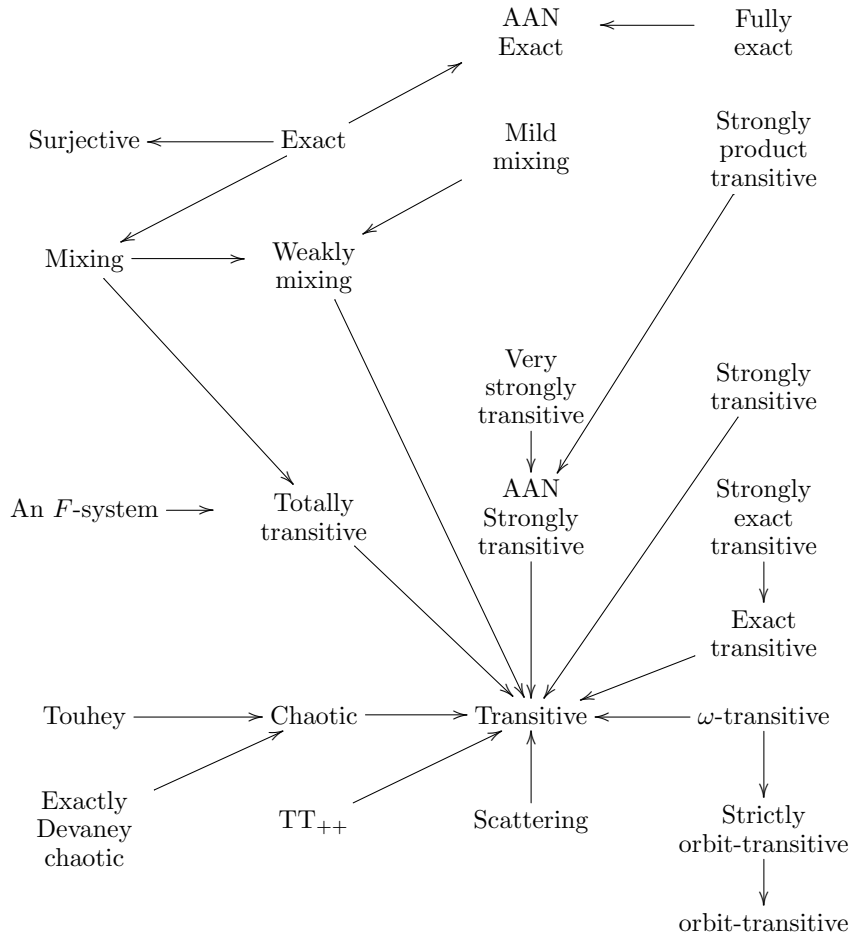
Figure: Inclusions between some classes of functions.
