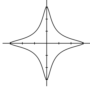
Edwardsova krivulja u^2 + v^2 = 9(1 - u^2 v^2)
